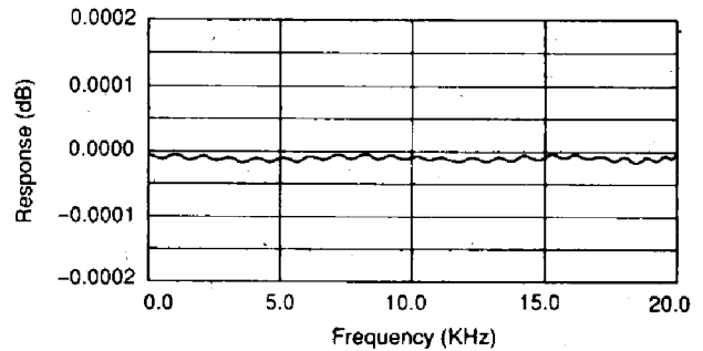
Ripple characteristics
