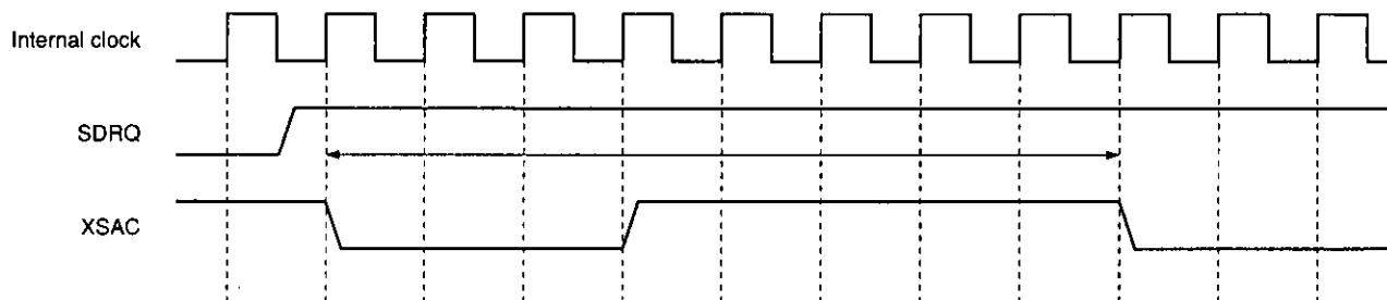
XFRRATE [1:0] = 3
