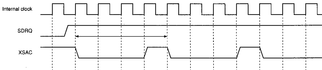
XFRRATE [1:0] = 0
