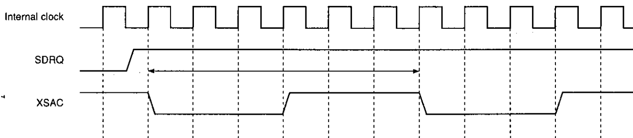
XFRRATE [1:0] = 1
