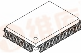
CXD1812Q 100 pin QFP (Plastic)
