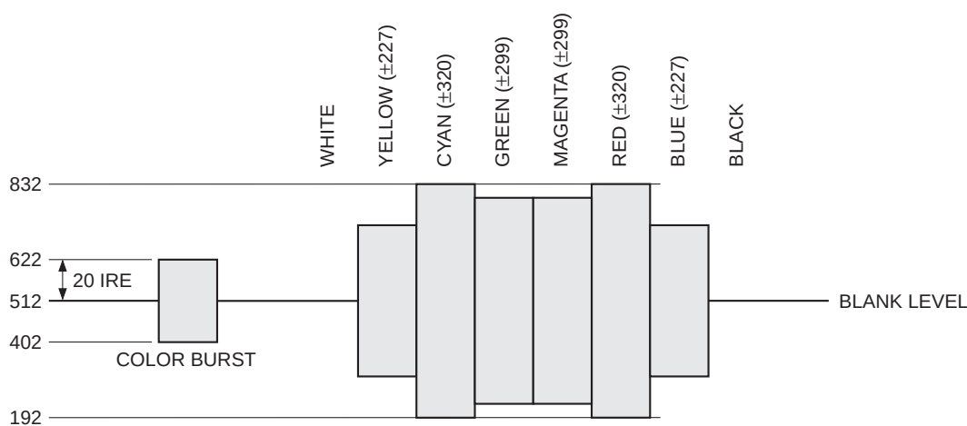
NTSC C (chroma) signal output waveform 7.5 IRE setup
