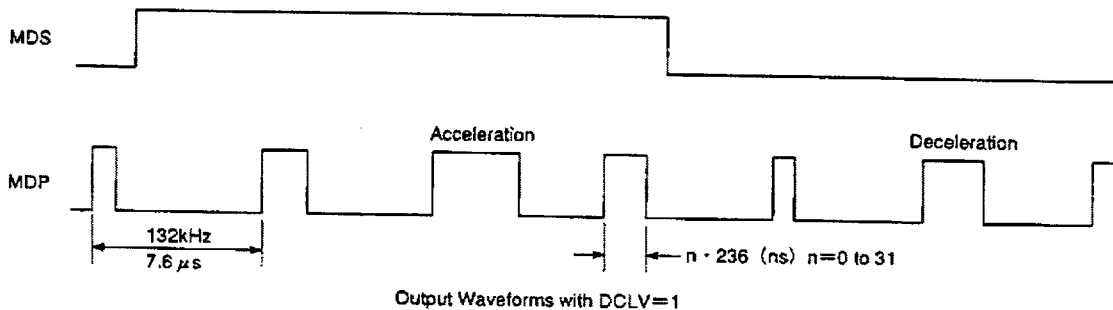
Output Waveforms with DCLV=1
