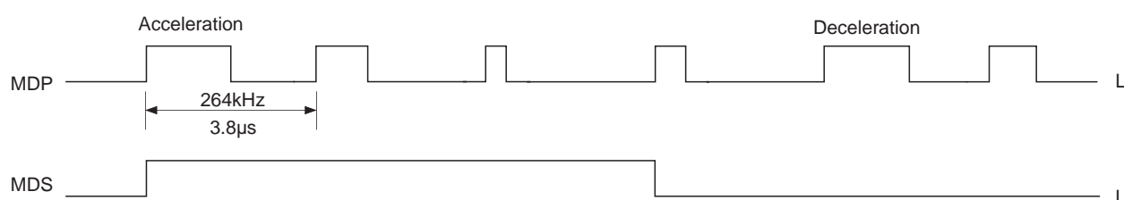
Timing Chart 1-26
