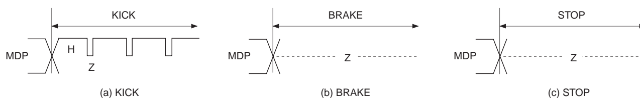
Timing Chart 1-9
