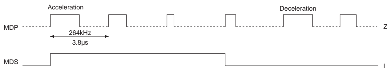
Timing Chart 1-36
