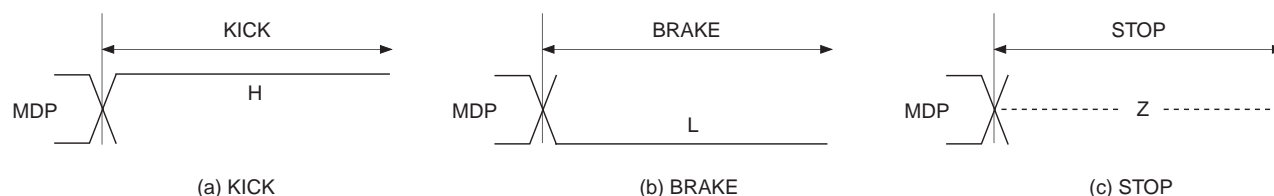
Timing Chart 1-10
