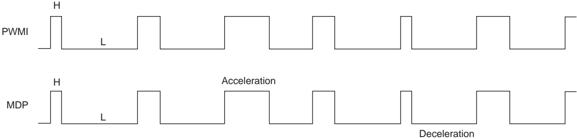
Timing Chart 1-17
