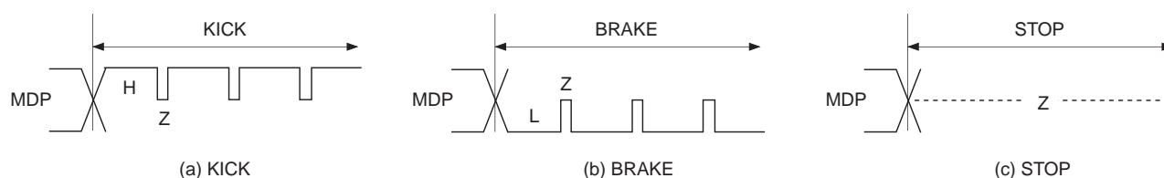
Timing Chart 1-8
