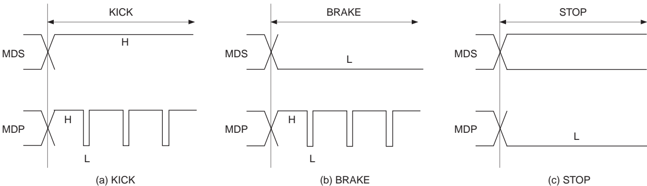
Timing Chart 1-19
