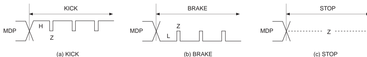
Timing Chart 1-7
