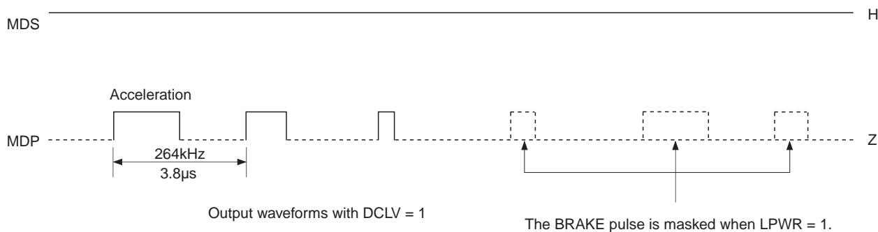
Timing Chart 1-35
