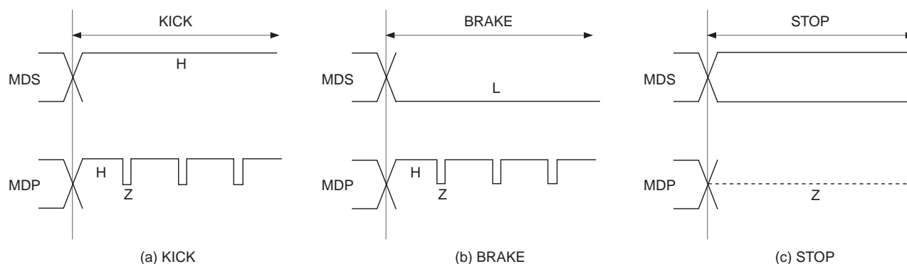
Timing Chart 1-31
