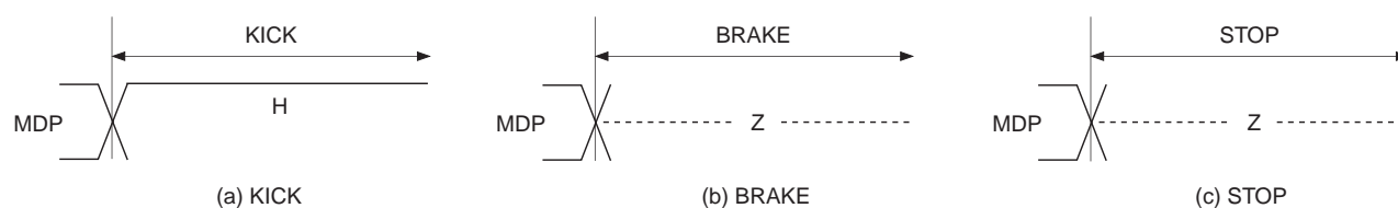
Timing Chart 1-10
