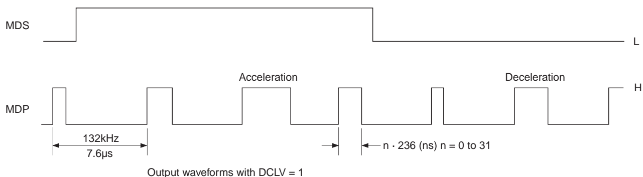
Timing Chart 1-24
