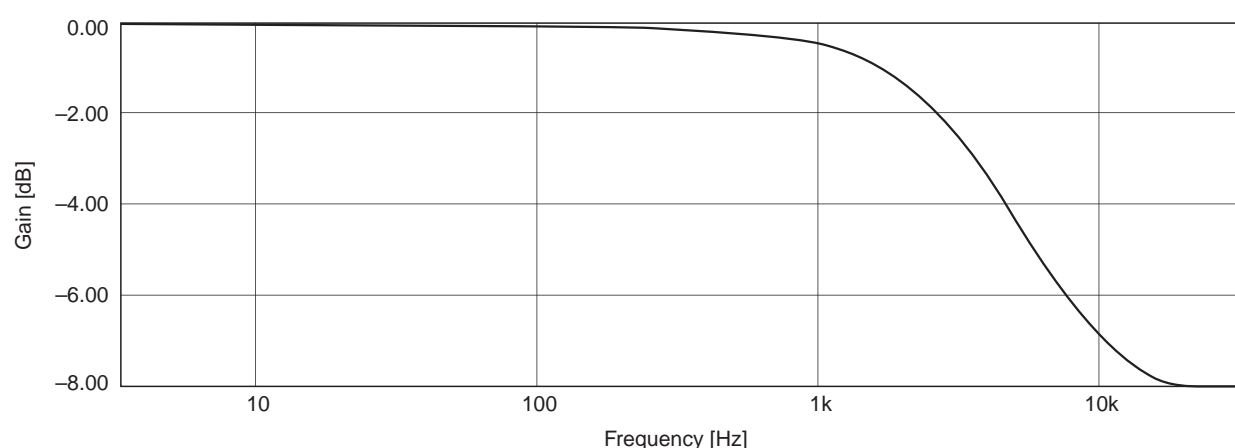
Fig. 4-14. High-Cut Filter Frequency Response
