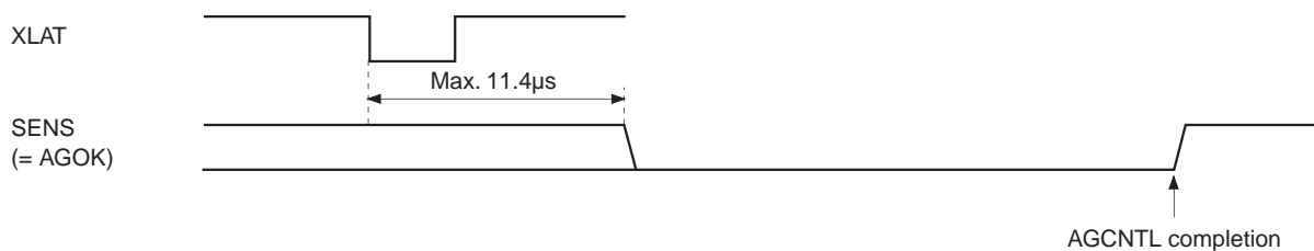
Timing Chart 5-4.
