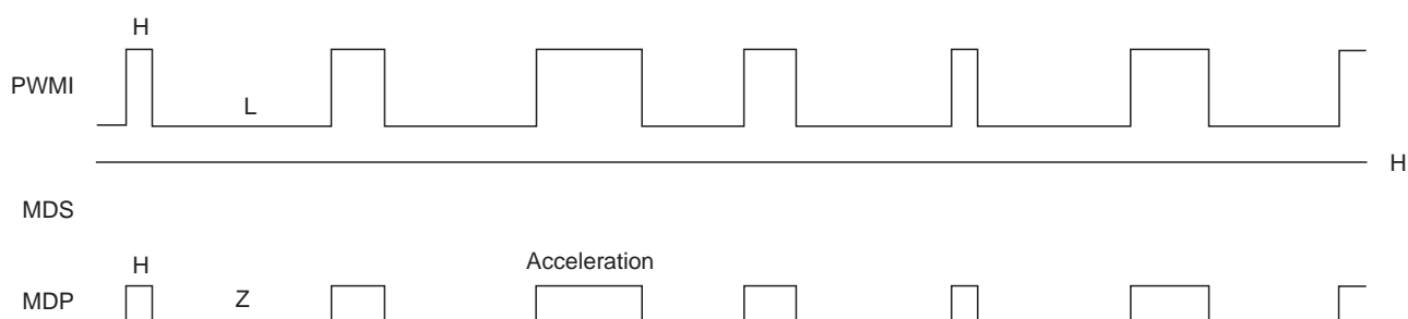
Timing Chart 1-39
