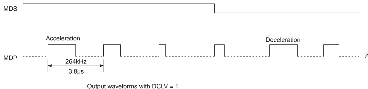
Timing Chart 1-35
