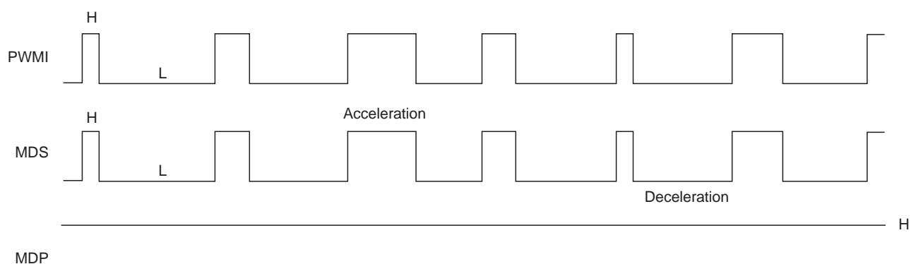
Timing Chart 1-39
