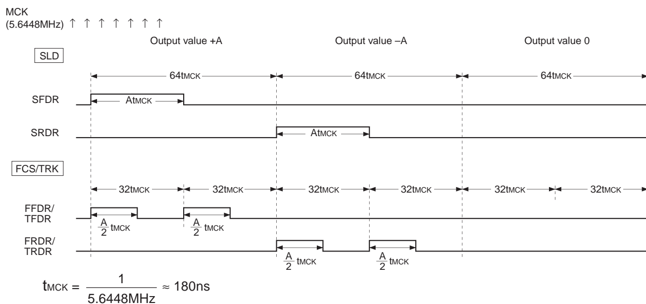
Timing Chart 5-20.
