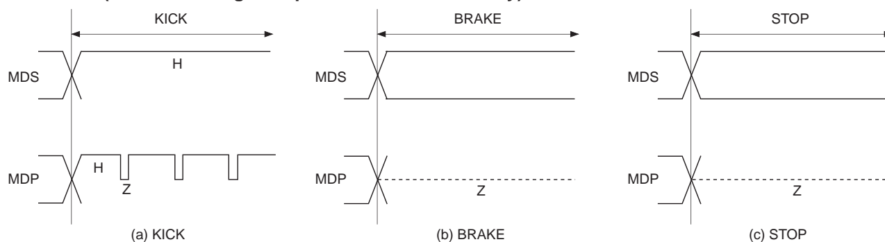
Timing Chart 1-32
