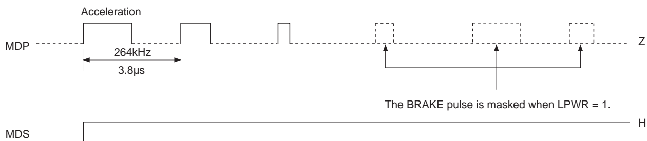
Timing Chart 1-38
