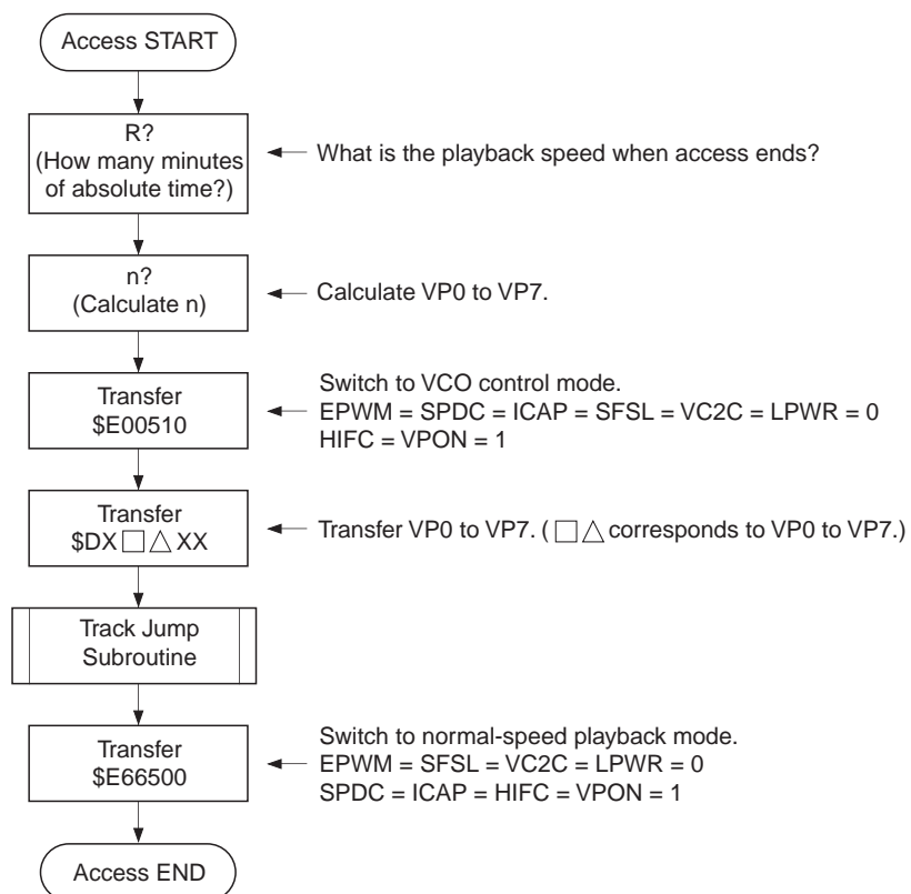
Fig. 3-3. Access Flow Chart Using VCO Control
