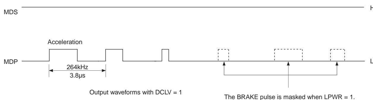
Timing Chart 1-25
