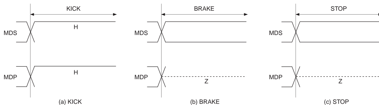
Timing Chart 1-33
