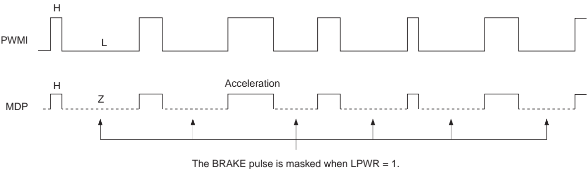
Timing Chart 1-17
