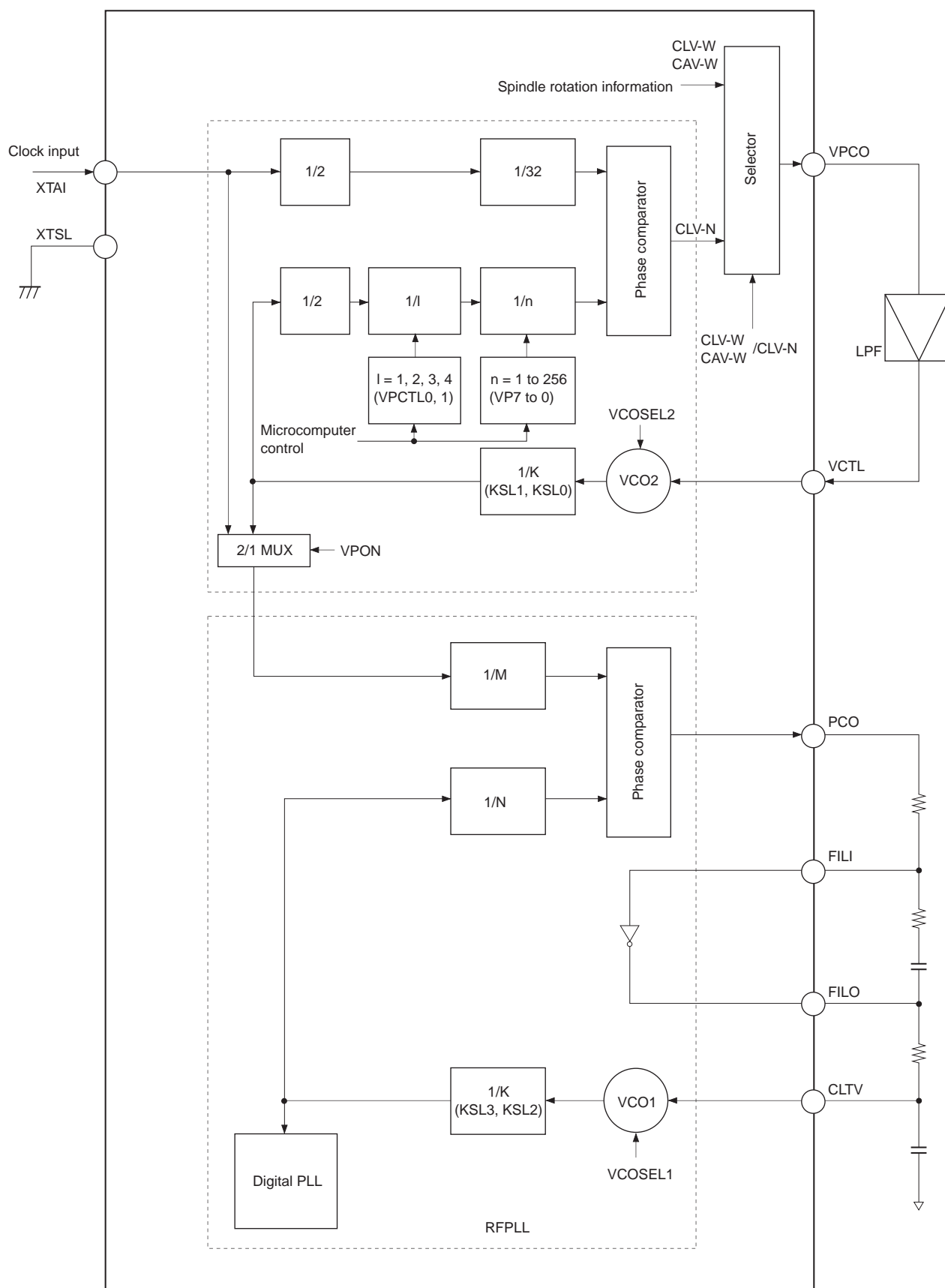
Block Diagram 4-1
