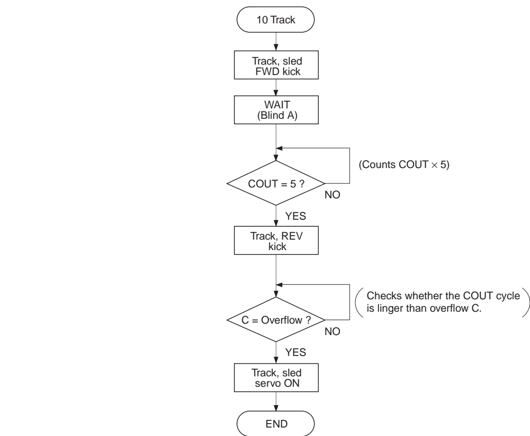
Fig. 4-8-(a). 10-Track Jump Flow Chart
