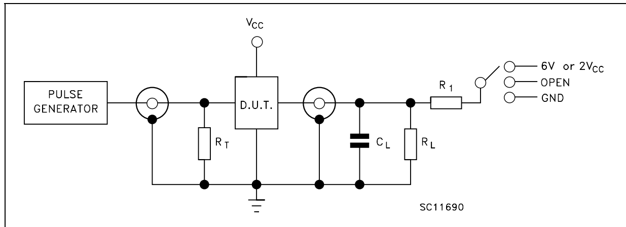
Figure 4: Test Circuit
