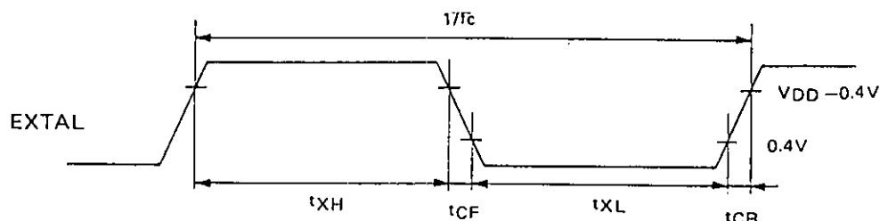
Fig. 1 Clock timing
