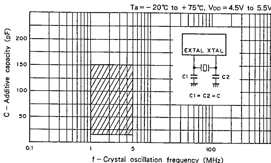
Fig. 10 Crystal oscillator circuit additive capacity calculation chart
