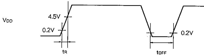
Fig. 11 Power on reset
