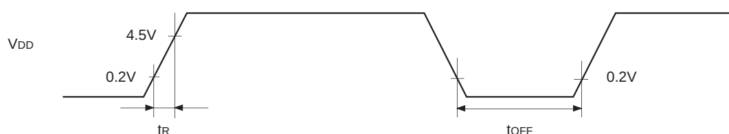
Fig. 8. Power-on reset
