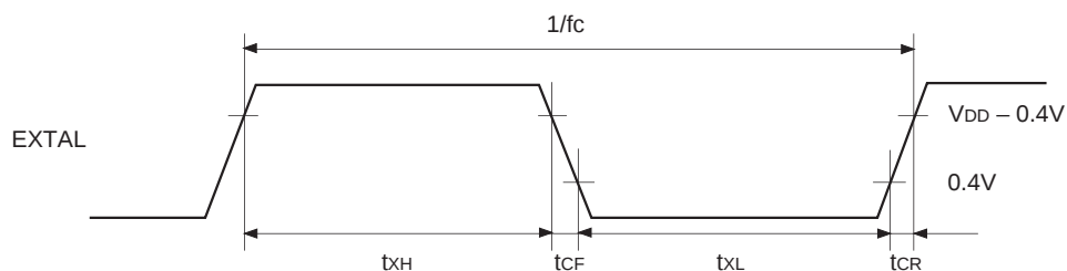
Fig. 1. Clock timing
