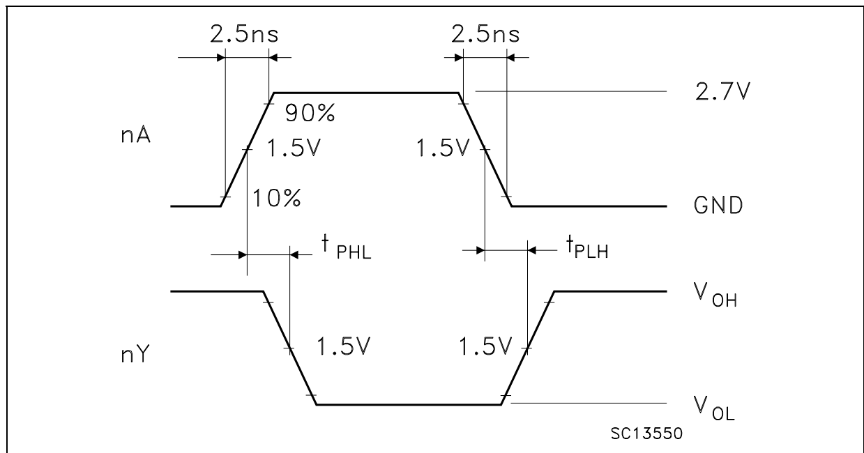
Figure 4: Waveform - Propagation Delay (f=1MHz; 50% duty cycle)
