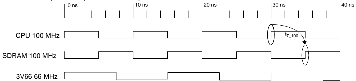
CPU to SRAM Skew, CPU leads SDRAM by 5.0 ns (500-ps window)
