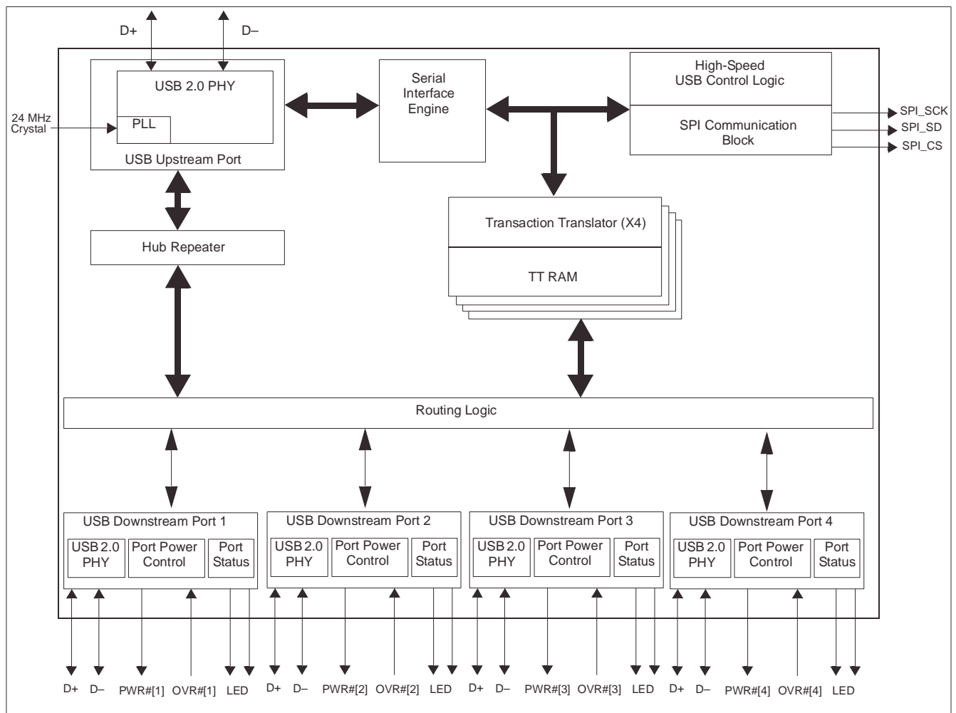
Figure 2-1. Block Diagram
