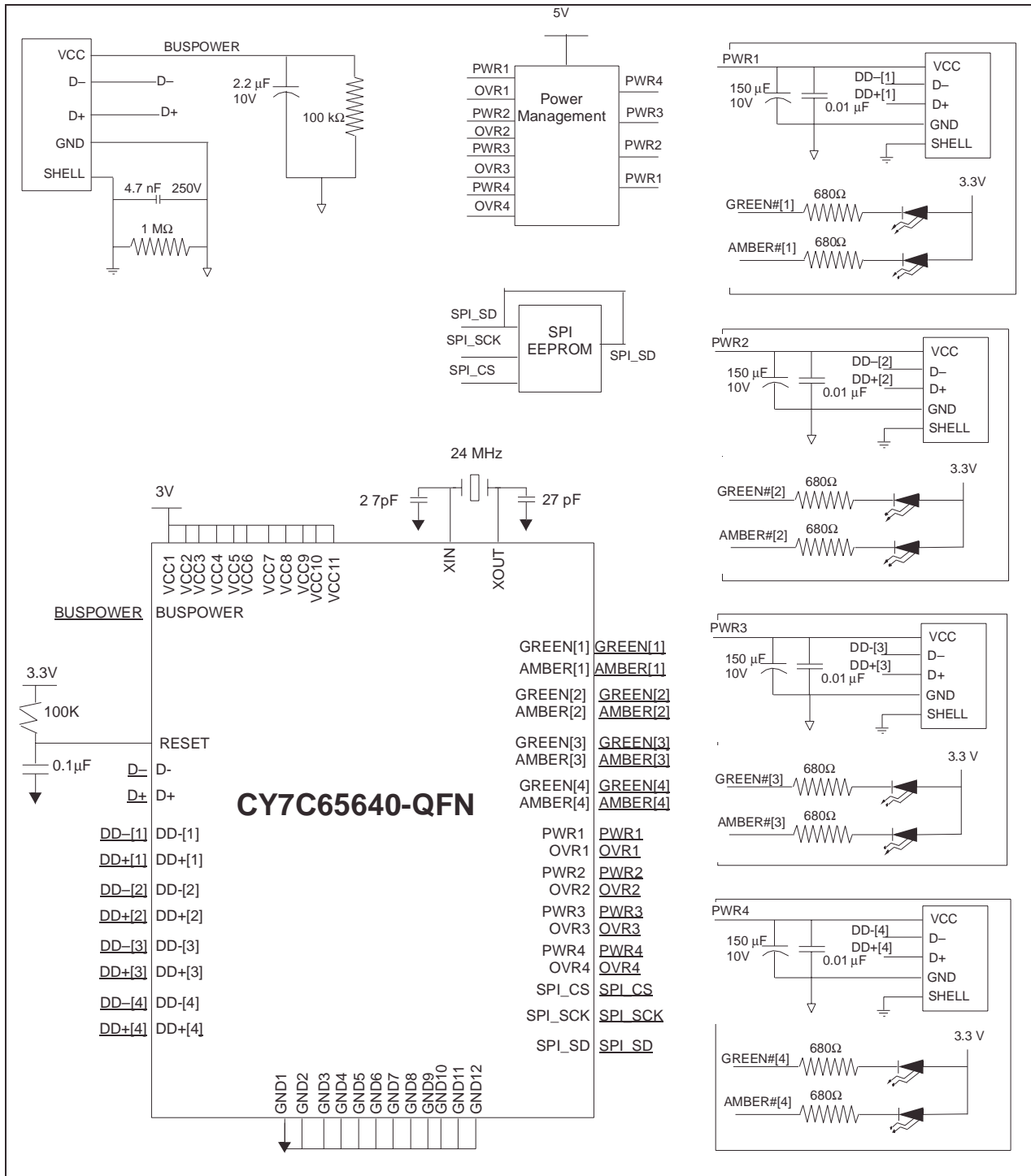
Figure 13-1. Sample Schematic
