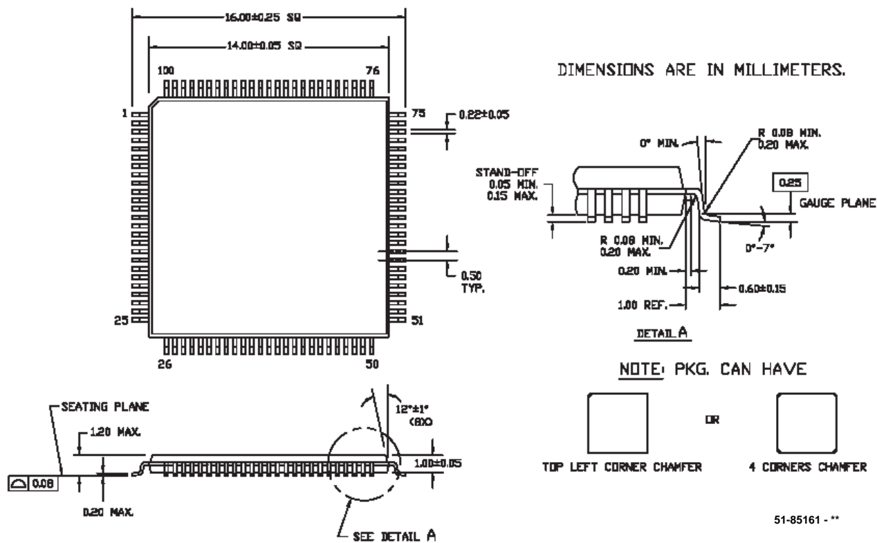
Figure 4-7. 100-Lead TQFP
