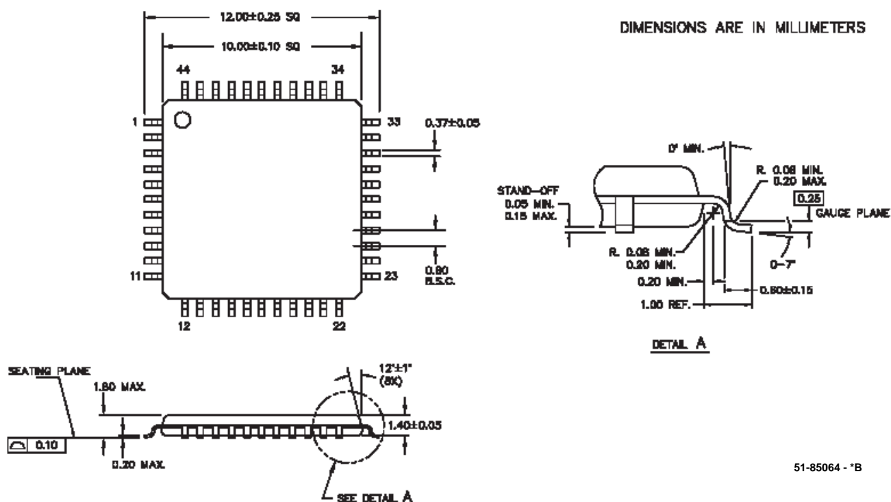
Figure 4-4. 44-Lead TQFP
