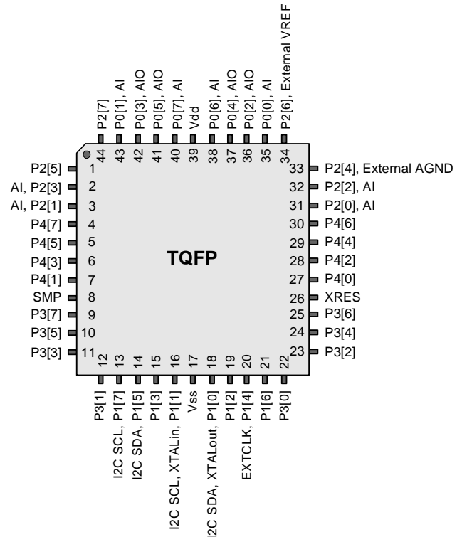
CY8C29566 44-Pin PSoC Device
