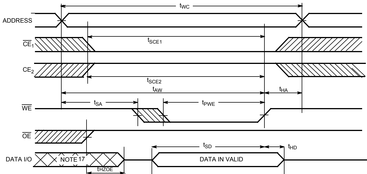
Write Cycle No. 1 ( \overline{WE} Controlled) [10, 15, 16]
