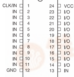
DIP/SOIC
