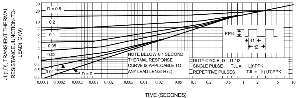
Fig. 3-TYPICAL THERMAL RESPONSE
