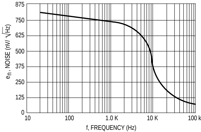
Figure 5. Noise Voltage
