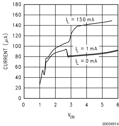
Ground Current vs V_{IN} @ 125°C
