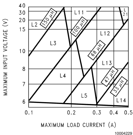
FIGURE 4. LM2671-3.3
