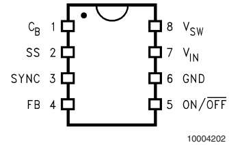
8-Lead Package Top View
