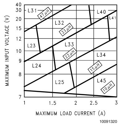
FIGURE 4. LM2673-5.0
