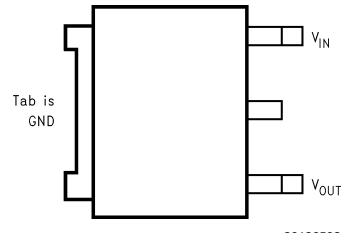
TO-252, Top View LP38691DT-X.X
