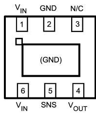
6-Lead LLP, Bottom View LP38691SD-X.X
