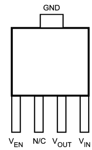
SOT-223, Top View LP38693MP-X.X
