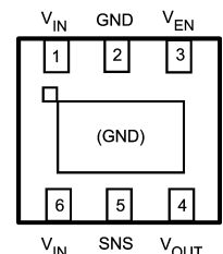
6-Lead LLP, Bottom View LP38693SD-X.X
