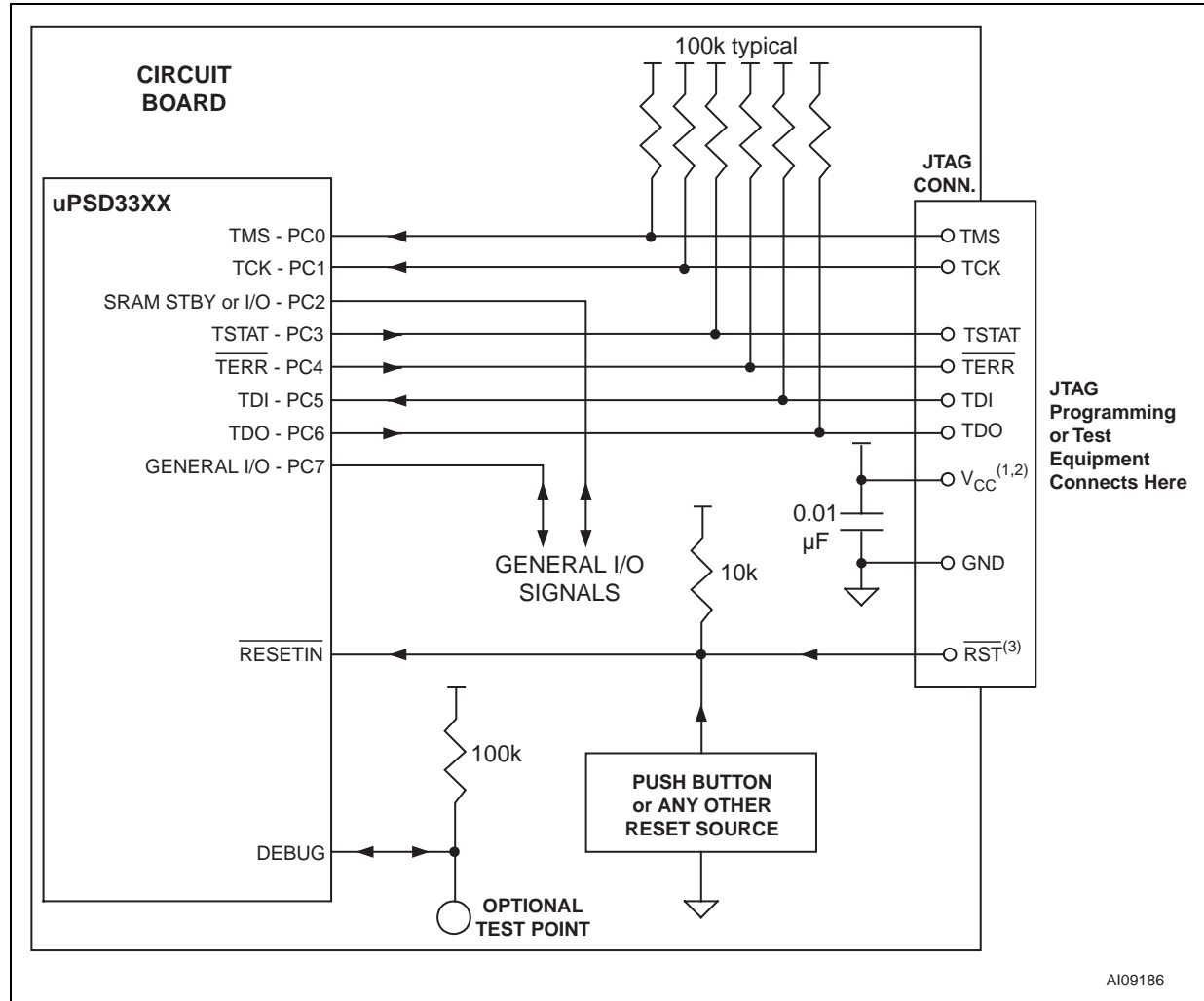
Figure 82. Recommended 6-pin JTAG Connections
