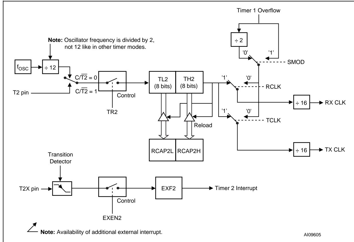
Figure 27. Timer 2 in Baud Rate Generator Mode
