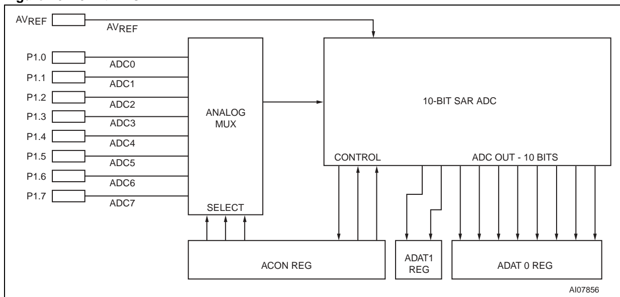
Figure 46. 10-Bit ADC
