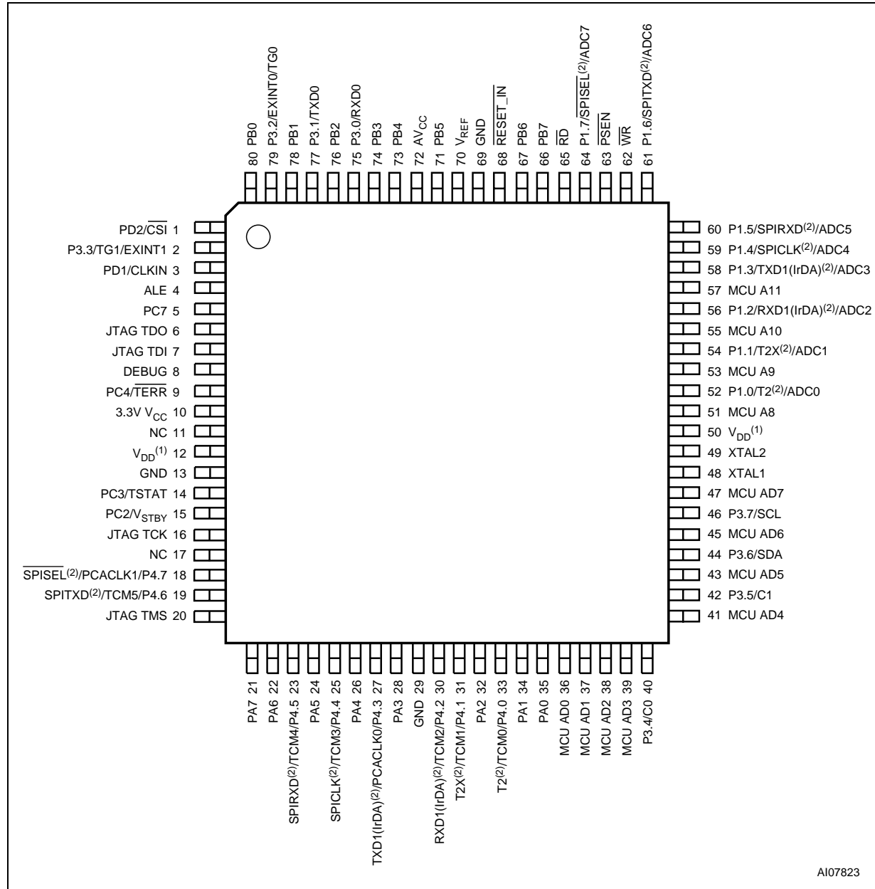
Figure 4. TQFP80 Connections
