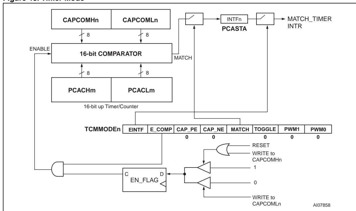
Figure 48. Timer Mode
