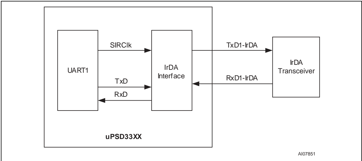
Figure 36. IrDA Interface
