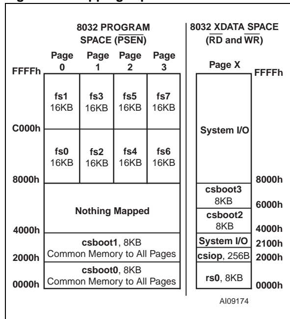
Figure 55. Mapping: Split Second Flash in Half
