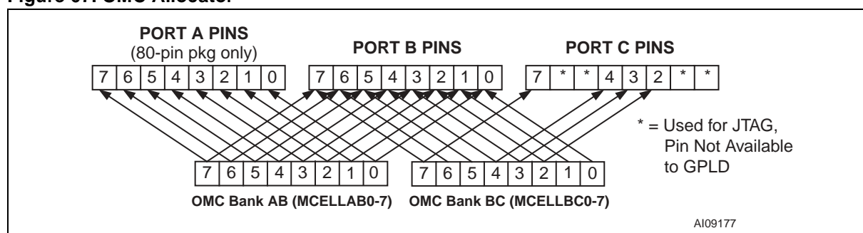
Figure 67. OMC Allocator
