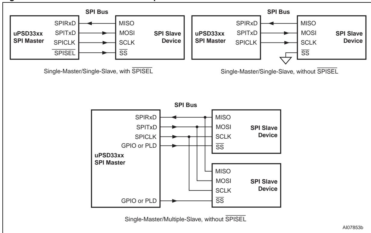
Figure 41. SPI Device Connection Examples
