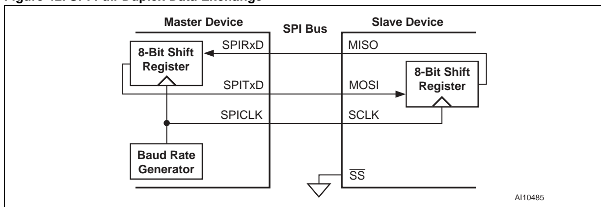
Figure 42. SPI Full-Duplex Data Exchange
