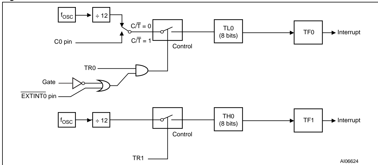
Figure 24. Timer/Counter Mode 3: Two 8-bit Counters
