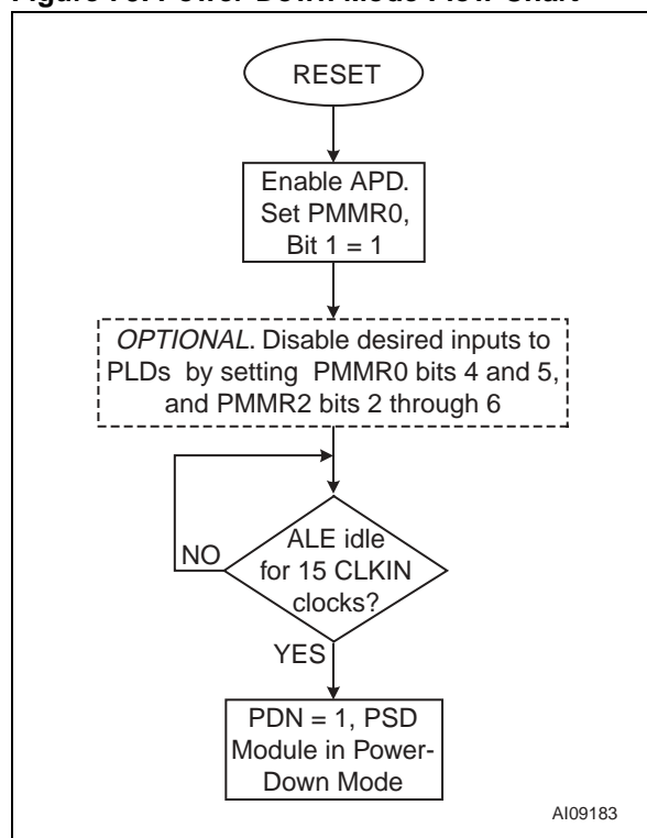
Figure 79. Power-Down Mode Flow Chart
