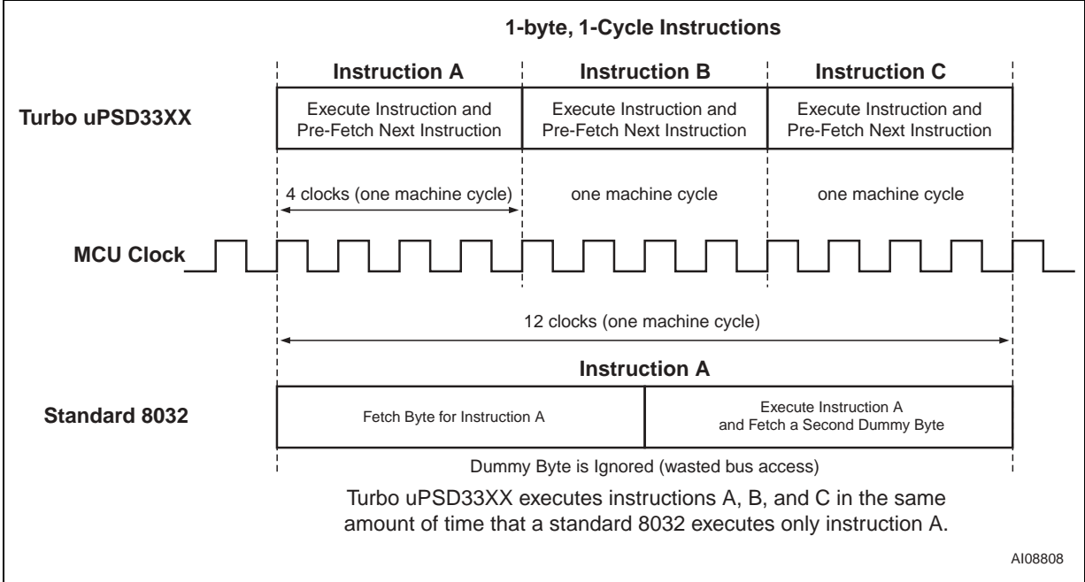
Figure 7. Comparison of uPSD33xx with Standard 8032 Performance
