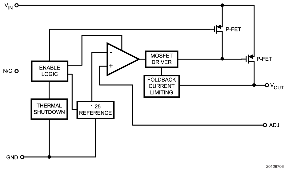
FIGURE 1. LP38690-ADJ Functional Diagram (LLP)
