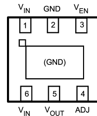
20126705 6-Lead LLP, Bottom View LP38692SD-ADJ
