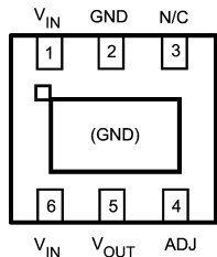
20126704 6-Lead LLP, Bottom View LP38690SD-ADJ
