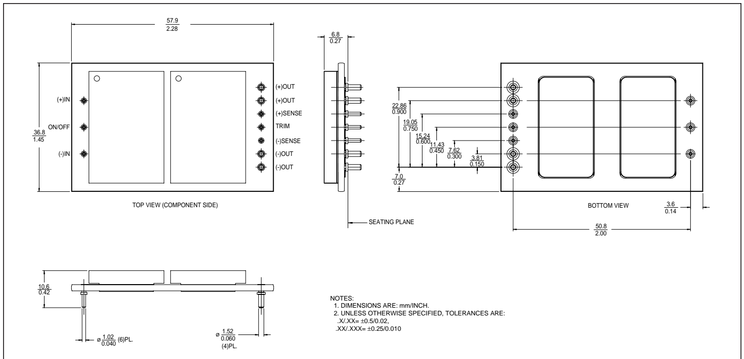
Figure 2— Mechanical outline and PCB footprint information; dual output pin version (package style 2)
