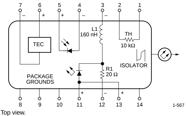
Figure 2. Circuit Schematic
