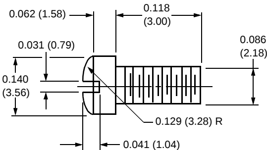
Note: Dimensions are in inches and (millimeters). 1-532(C)
