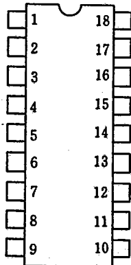
端子接続図/Connection Diagram (Top View)
