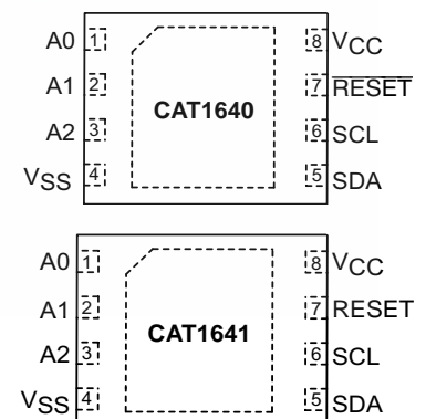
TDFN PACKAGE: 4.9MM X 3MM (RD2, ZD2)
