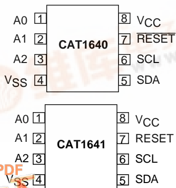
PDIP (P, L) SOIC (J, W)
