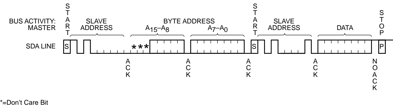
Figure 11. Selective Read Timing
