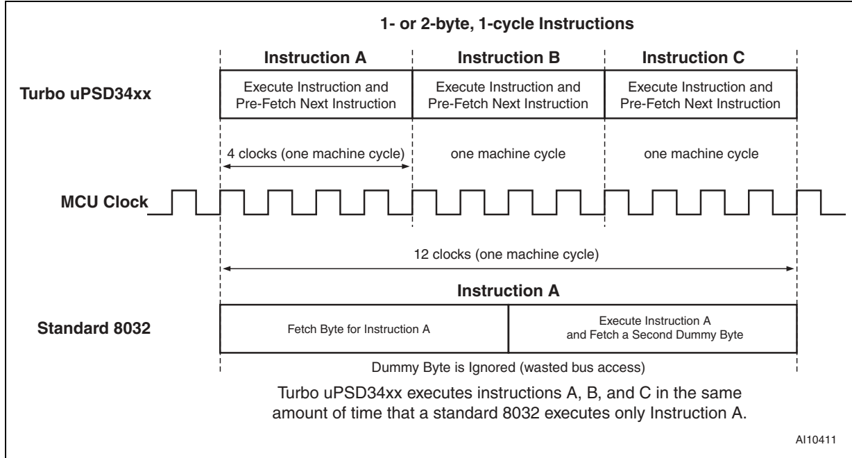
Figure 7. Comparison of uPSD34xx with Standard 8032 Performance
