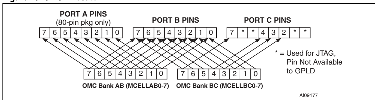
Figure 78. OMC Allocator
