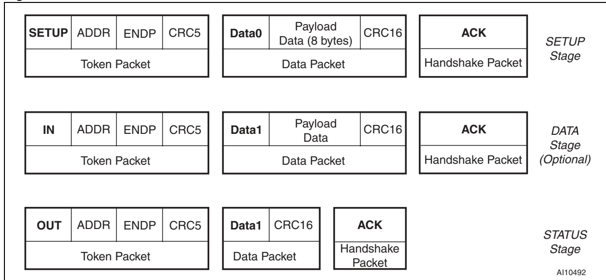
Figure 53. Control Transfer
