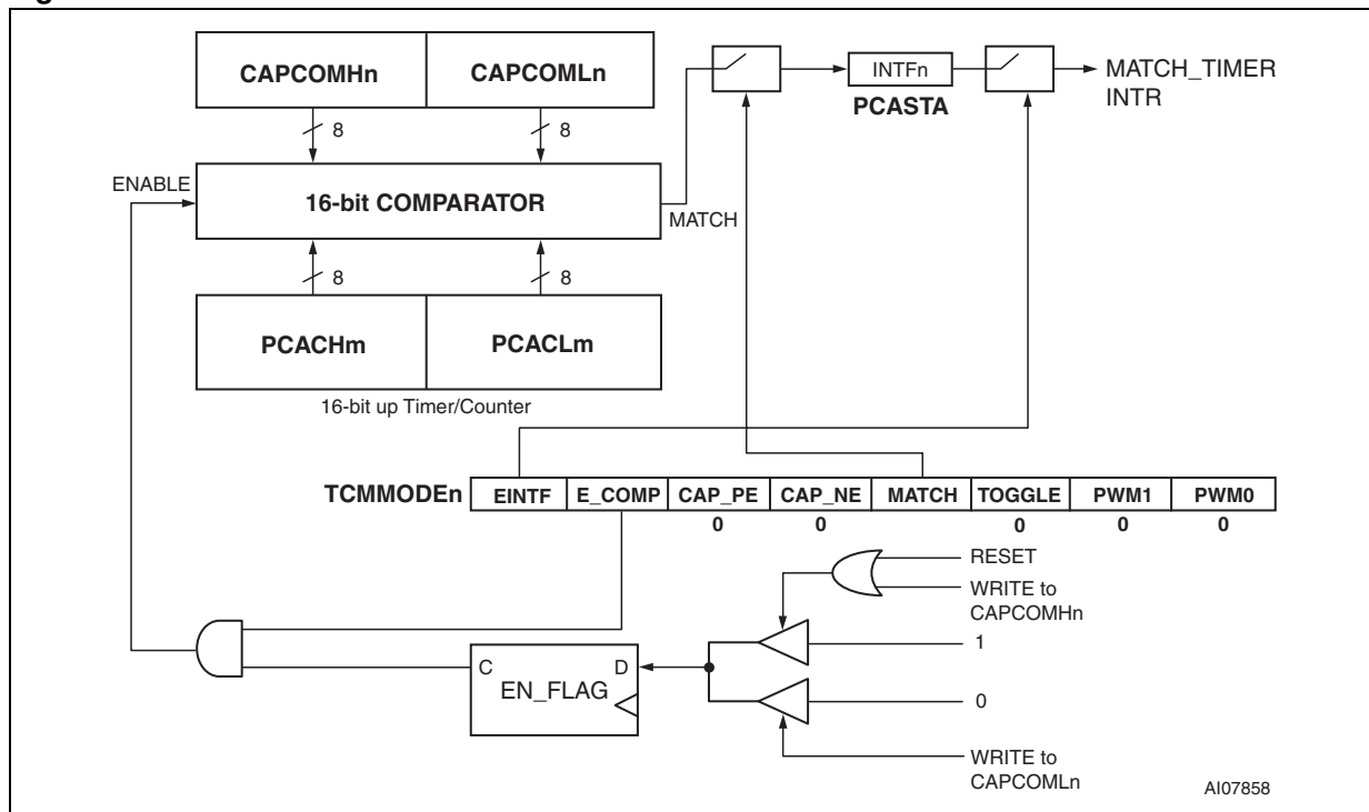
Figure 59. Timer Mode
