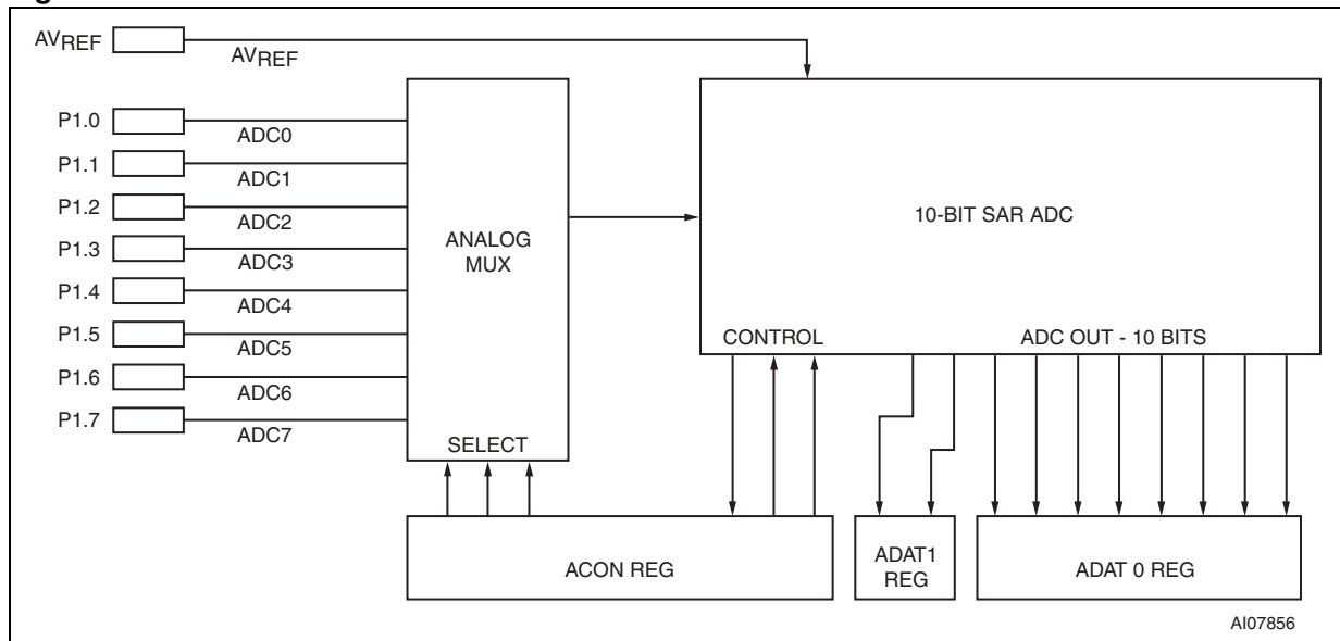
Figure 57. 10-Bit ADC
