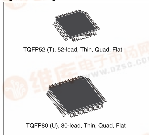
Figure 1. Packages
