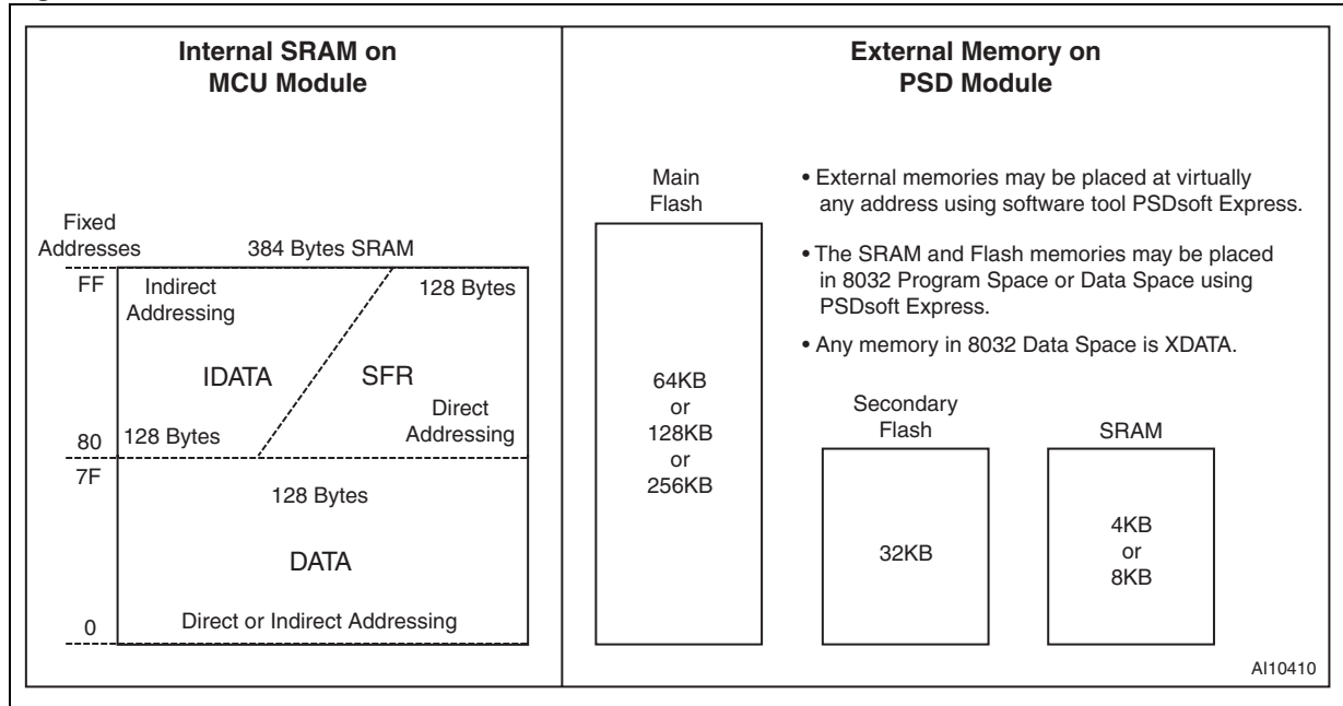
Figure 6. uPSD34xx Memories
