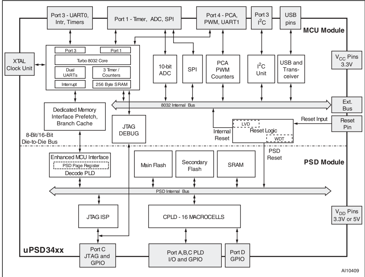
Figure 5. Functional Modules
