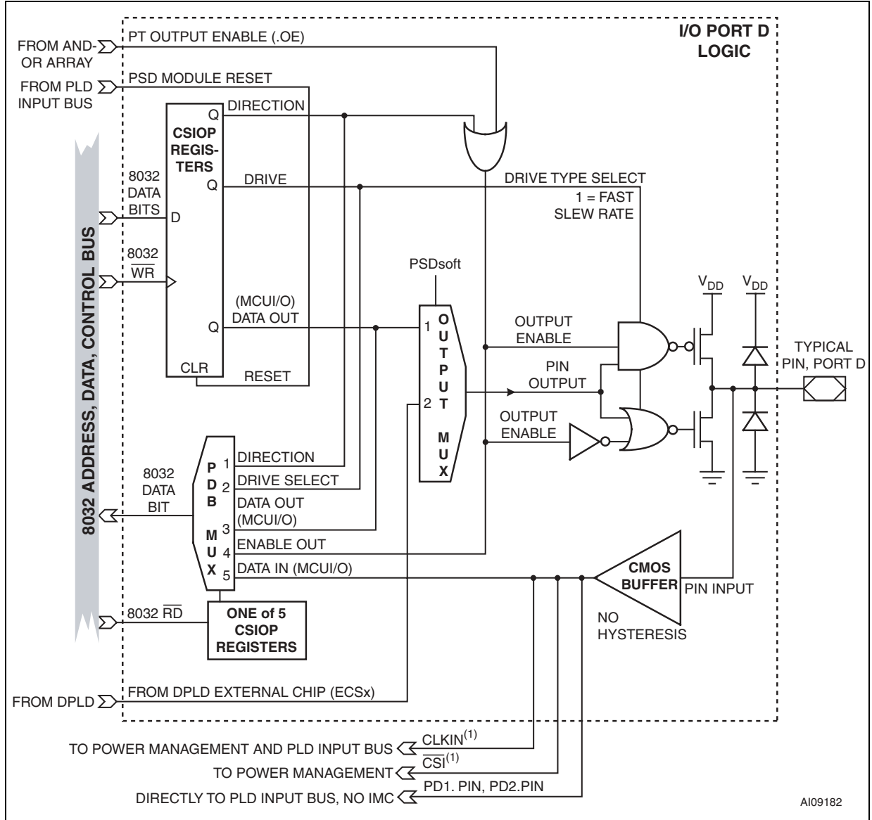
Figure 88. Port D Structure
