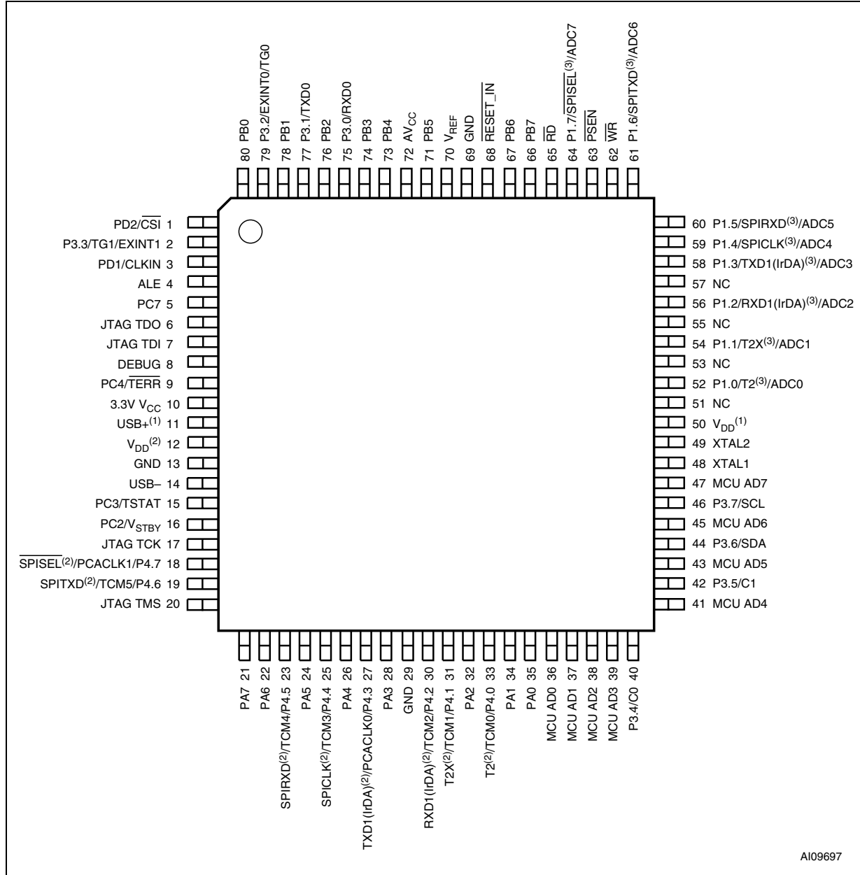
Figure 4. TQFP80 Connections
