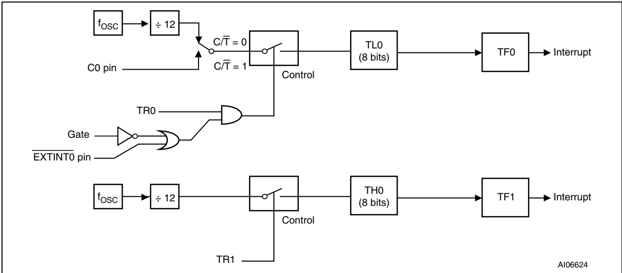
Figure 27. Timer/Counter Mode 3: Two 8-bit Counters
