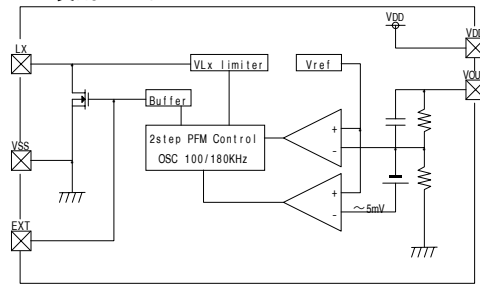
(2) XC6383E及XC6383F
