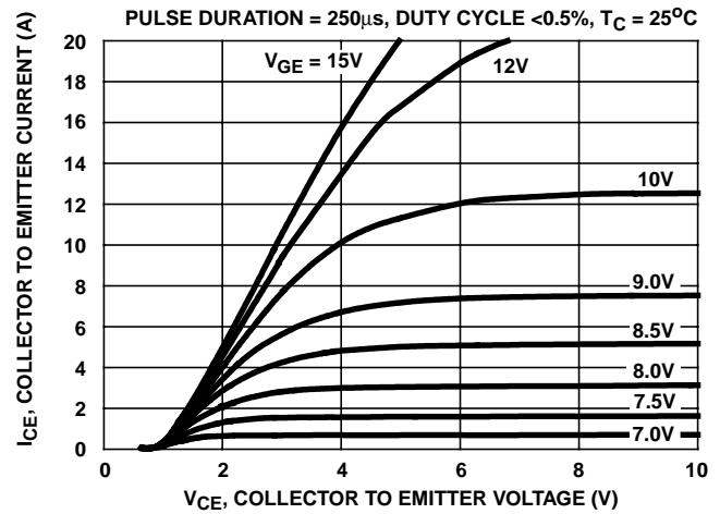
FIGURE 2. SATURATION CHARACTERISTICS
