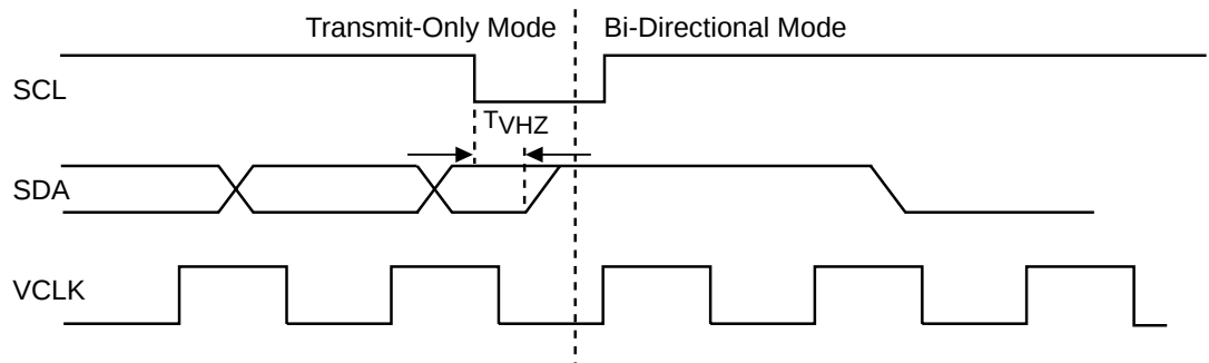
Figure 1. Mode Transition
