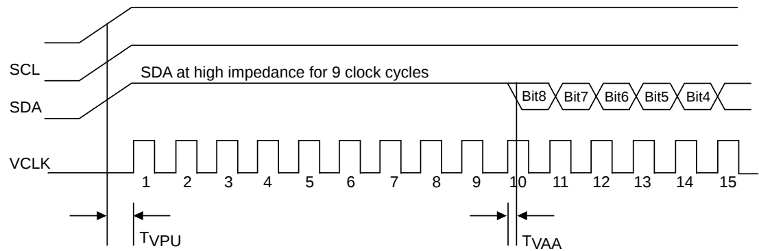
Figure 2. Device Initialization for Transmit-only Mode
