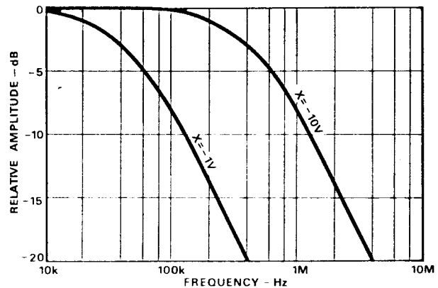
Figure 7. Typical Divide Mode Frequency Response
