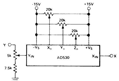
Figure 1. AD530 Functional Diagram.
