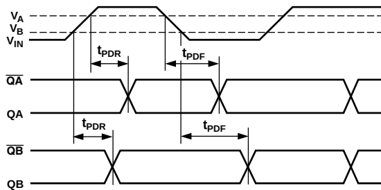
Figure 2. Timing Diagram 1
