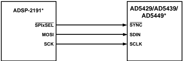
Figure 47. ADSP-2191 SPI to AD5429/AD5439/AD5449 Interface
