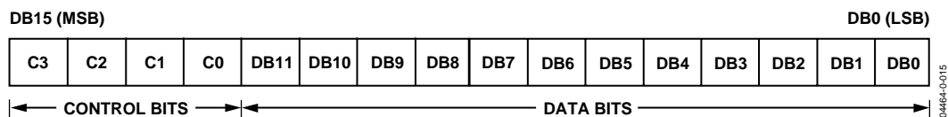
Figure 45. AD5449 12-Bit Input Shift Register Contents
