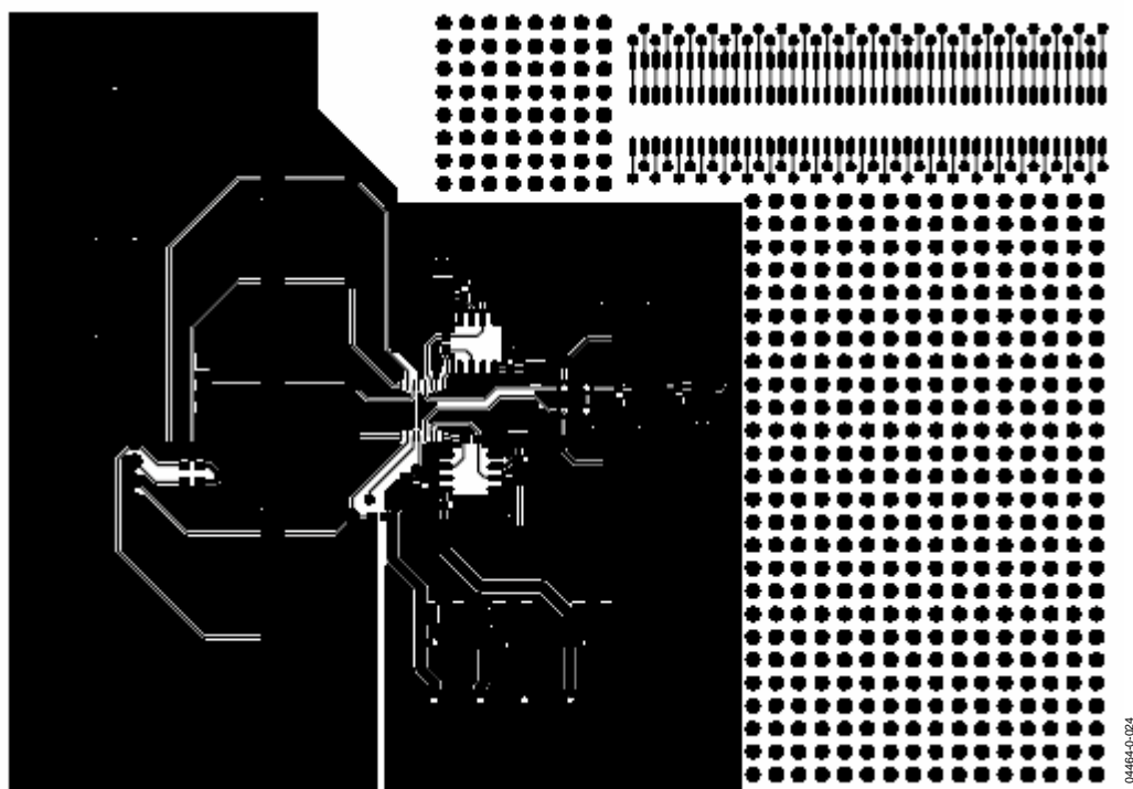
Figure 54. Component-Side Artwork
