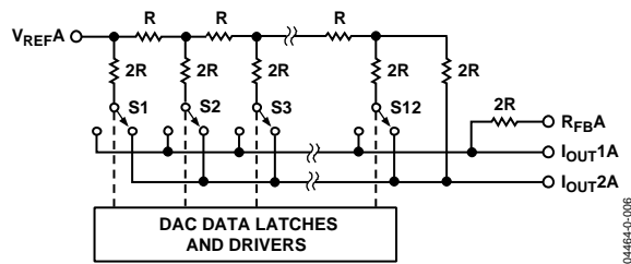
Figure 36. Simplified Ladder
