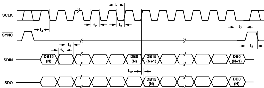
Figure 3. Daisy-Chain and Readback Modes Timing Diagram
