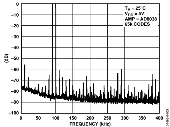
Figure 34. Wideband IMD, f_{OUT} = 90\text{ kHz} , 100 kHz, Clock = 25 MHz
