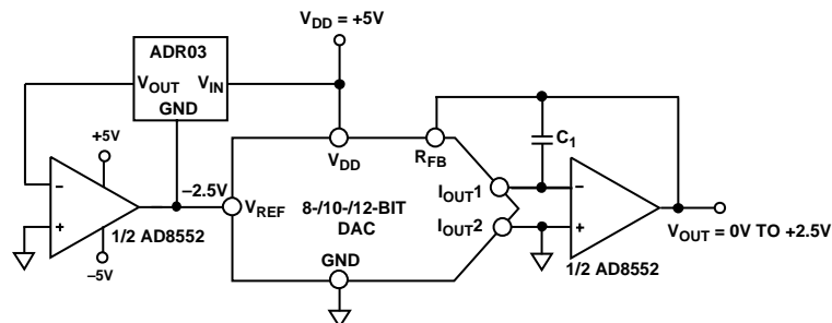
Figure 39. Single-Supply Voltage-Switching Mode
