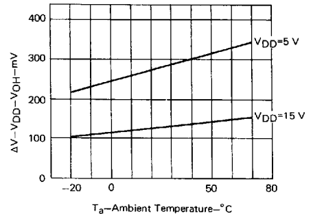
V_{DD} -OUTPUT HIGH VOLTAGE
