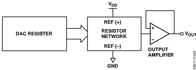
Figure 24. DAC Architecture
