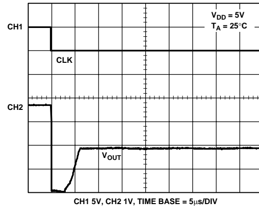
Figure 20. Exiting Power-Down
