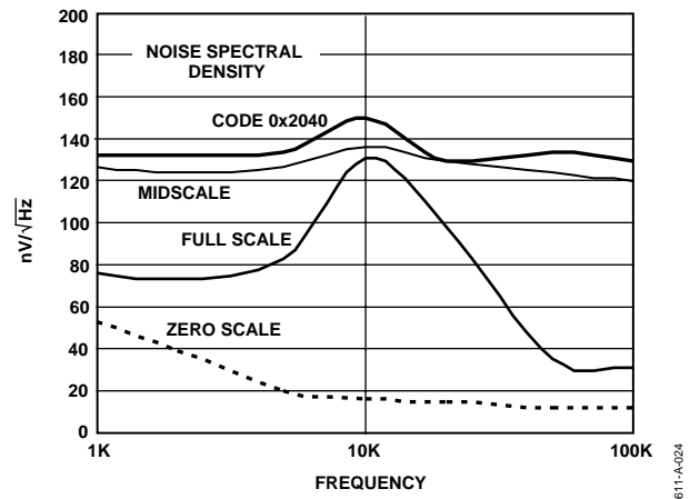
Figure 23. Noise Spectral Density
