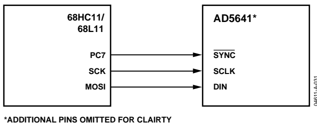
Figure 30. AD5641 to 68HC11/68L11 Interface
