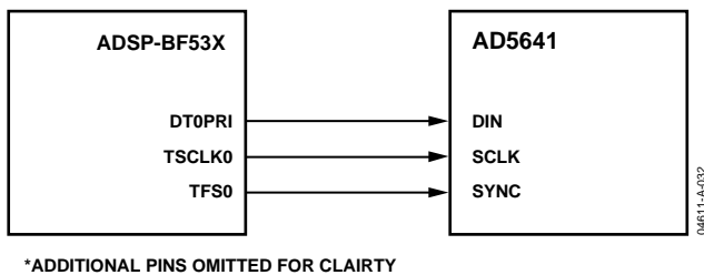
Figure 31. AD5641 to Blackfin ADSP-BF53X Interface
