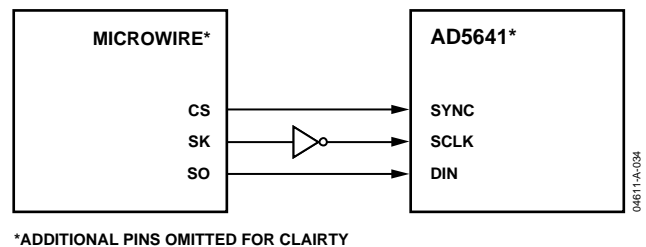
Figure 33. AD5641 to MICROWIRE Interface
