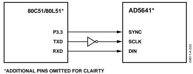
Figure 32. AD5641 to 80C51/80L51 Interface
