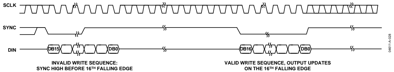
Figure 27. SYNC Interrupt Facility
