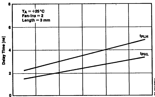
Delay Time vs Fan-Outs [NAND]
