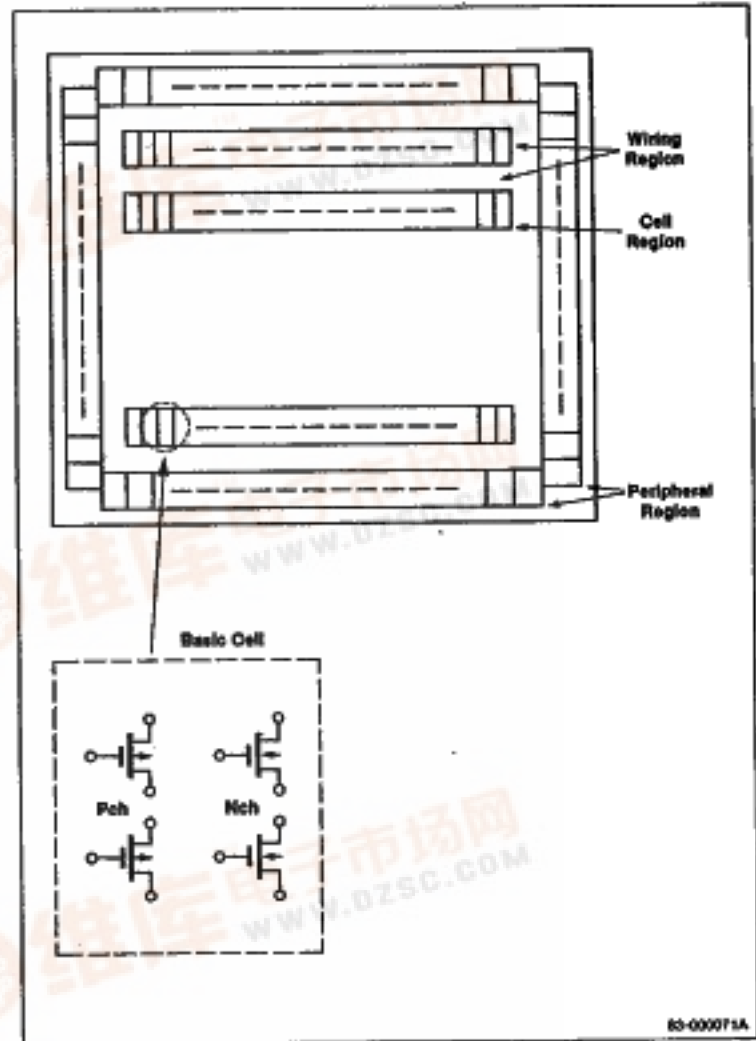
Figure 1. CMOS Gate Array Chip Layout
