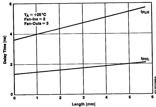
Delay Time vs Length [NOR]
