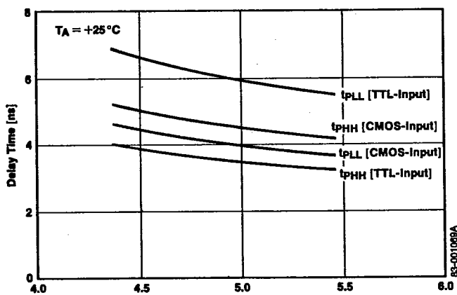
Delay Time vs Supply Voltage [Input Buffer]
