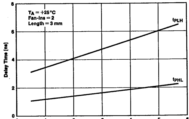
Delay Time vs Fan-Outs [NOR]
