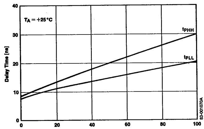
Delay Time vs Load Capacitance [Output Buffer]
