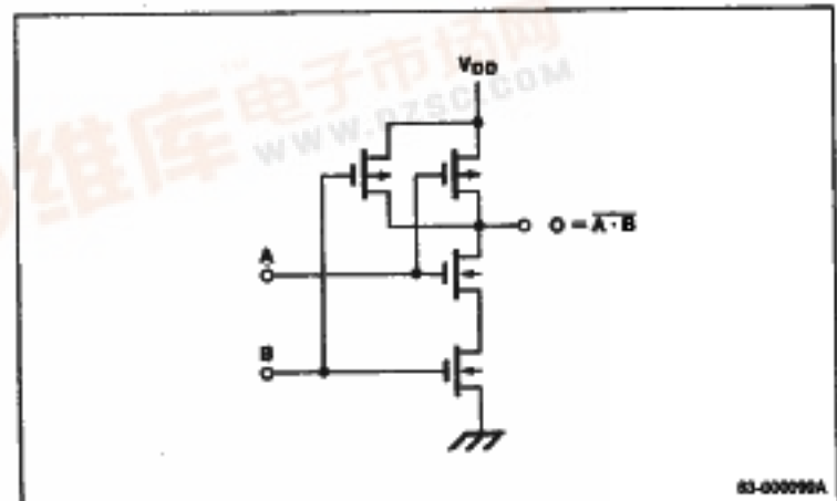
Figure 2. Cell Configured as a Two-Input NAND Gate
