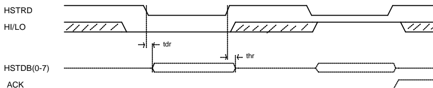
Figure 6. Host Interface D6571E - 8051
