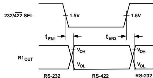
Figure 6. RS-232/RS-422 Receiver Enable Timing
