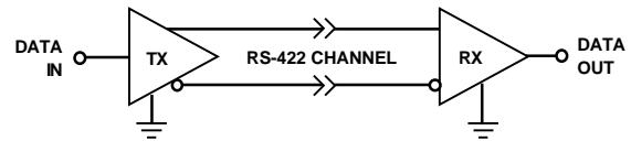
Figure 15. Differential RS-422 Interface
