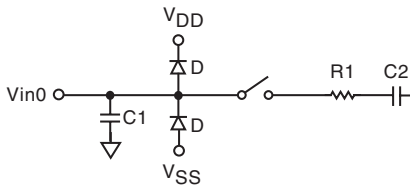
Figure 10. Equivalent Analog Input Circuit-(Single Ended)
