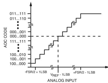
Figure 8. Twos Complement Transfer Characteristic (Bipolar Ranges)
