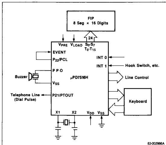
Figure 2. Telephone Application
