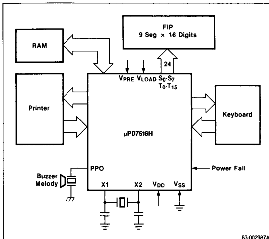
Figure 3. ECR Application
