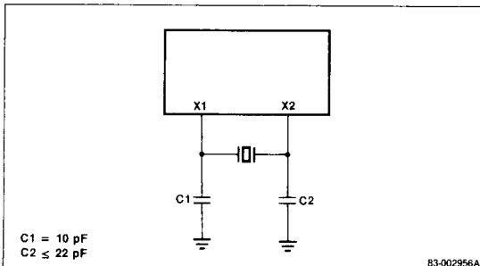
Figure 19. Crystal
