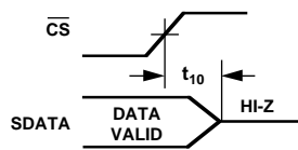
Figure 4. SSC Mode Data Hold Time
