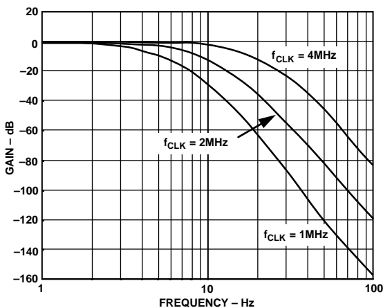
Figure 9. Frequency Response of AD7703 Filter
