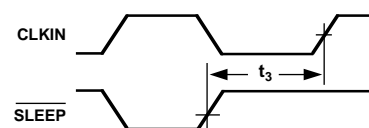
Figure 3. Sleep Mode Timing
