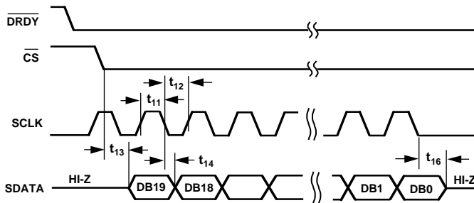
Figure 5b. SEC Mode Timing Diagram
