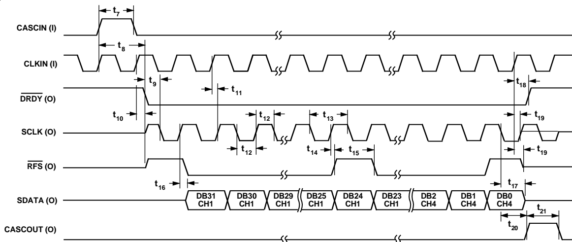
Figure 3. Master Mode Timing Diagram
