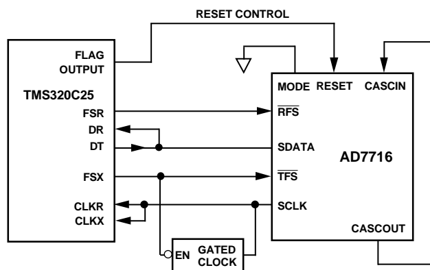
Figure 11. TMS320C25 to AD7716 Interface
