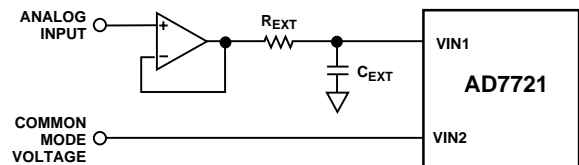
Figure 6. Antialiasing Circuits
