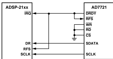
Figure 13. AD7721 to ADSP-21xx Interface
