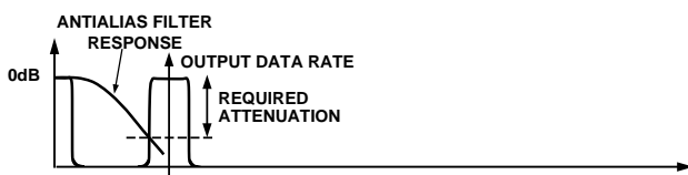
c. Frequency Response of Antialias Filter (Traditional ADC)
