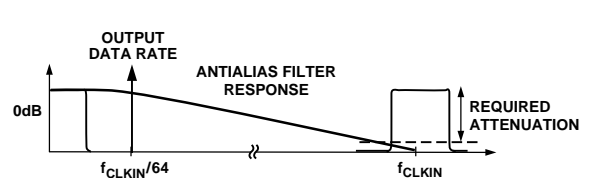
Figure 25b. Frequency Response of Antialias Filter
