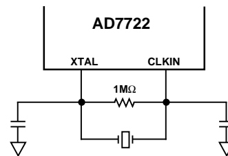
Figure 36. Crystal Oscillator Connection
