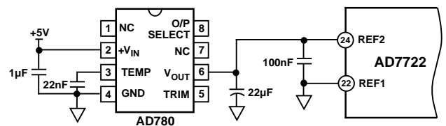
Figure 33. External Reference Circuit Connection
