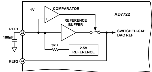
Figure 31. Reference Circuit Block Diagram
