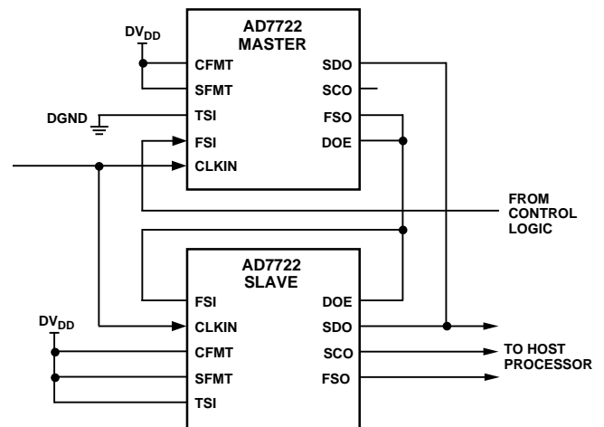
Figure 39. Connection for Two Channel Multiplexed Operation
