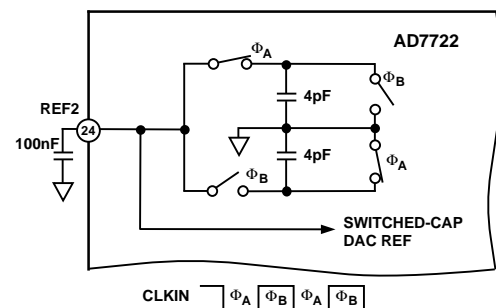
Figure 32. REF2 Equivalent Input Circuit
