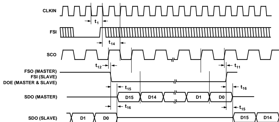
Figure 40. Timing for Two Channel Multiplexed Operation
