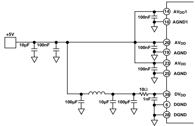
Figure 44. Power Supply Decoupling
