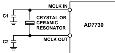
Figure 17. Crystal/Resonator Connections
