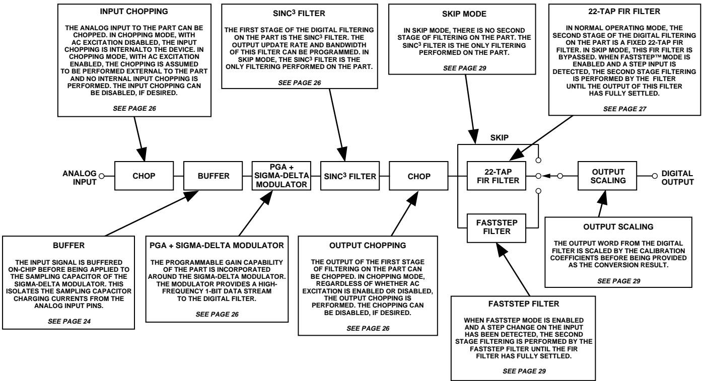
Figure 3. Signal Processing Chain
