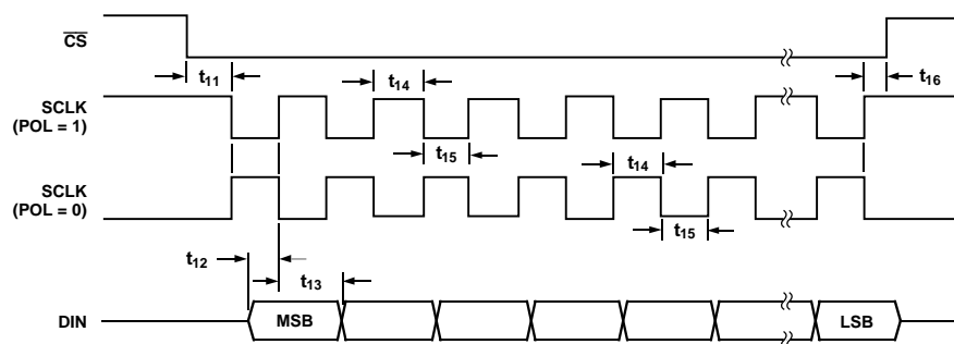
Figure 16. Write Cycle Timing Diagram
