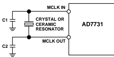
Figure 15. Crystal/Resonator Connections
