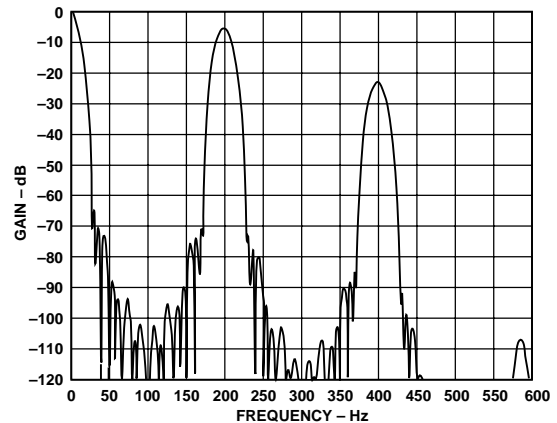
Figure 10. Expanded Full Frequency Response of AD7731 (SKIP = 0, CHP = 1, SF = 512)
