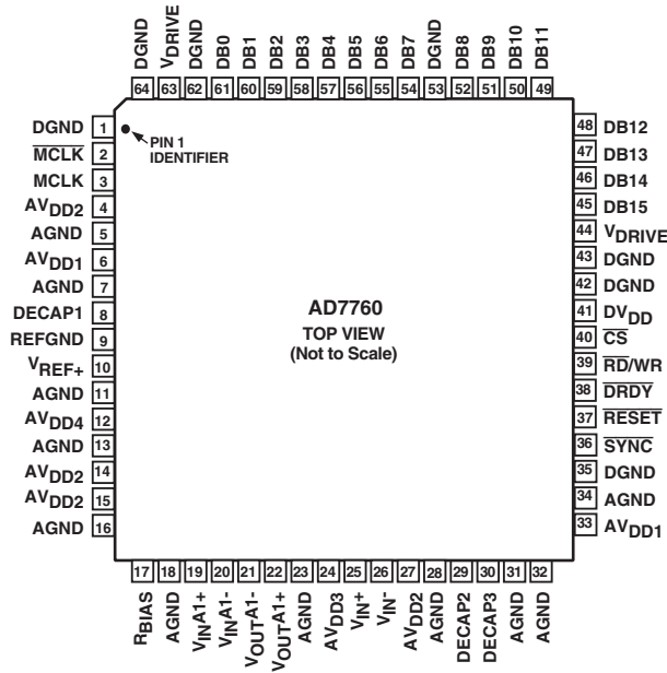
Figure 5. 64-Lead TQFP Pin Configuration
